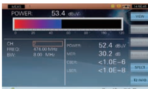
DVB-T2 signal measurement
