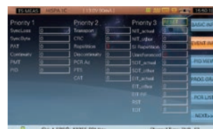
TR101 290 Three Level Monitoring
