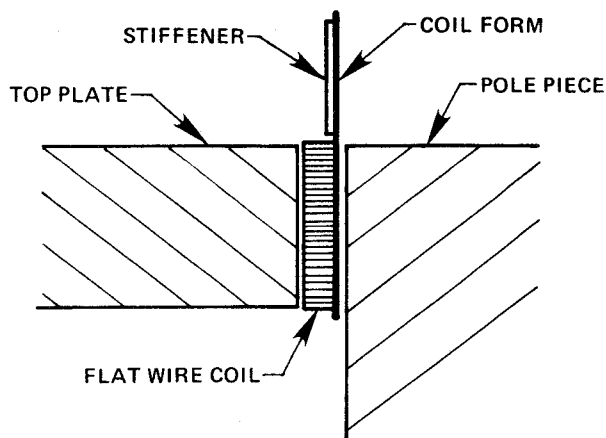
FIGURE 5 – Gap Structure
