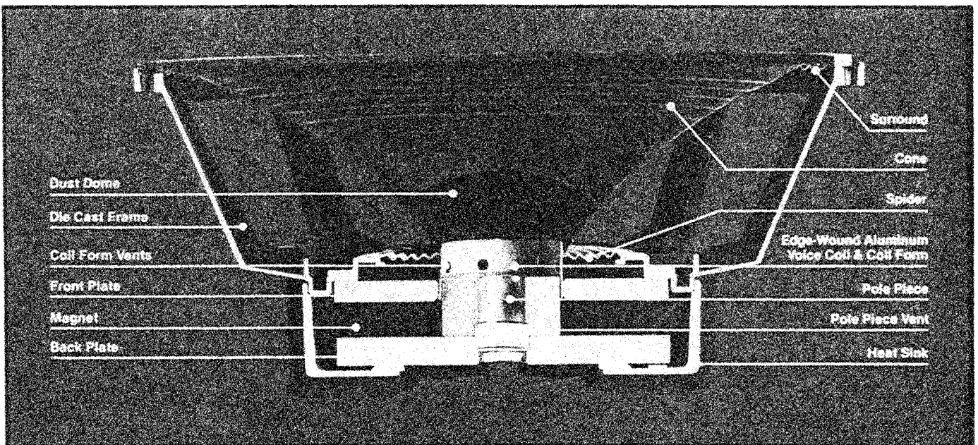
FIGURE 7 - EVM Cutaway
