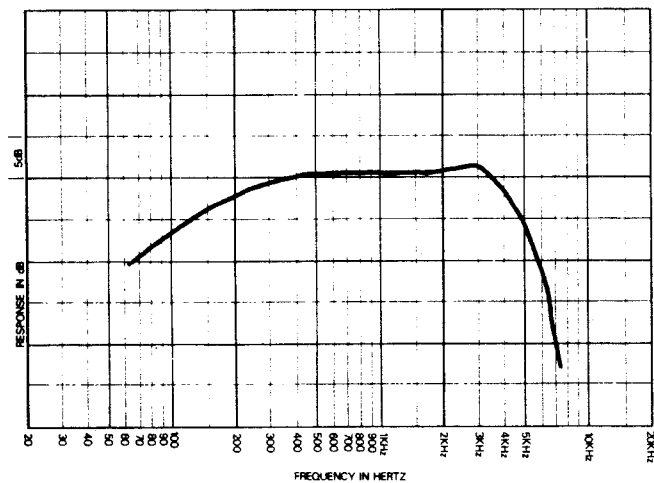
FIGURE 4 – Large Coil (4 in.) 12 in. Guitar Speaker
