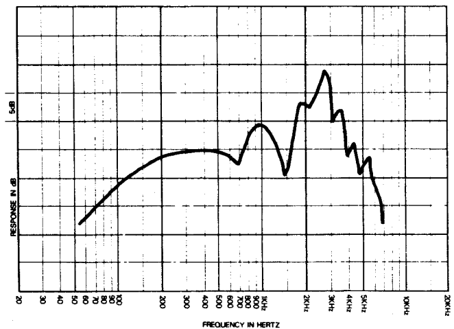
FIGURE 2 Inexpensive Small Coil 12 in. Guitar Speaker with Flat, Folded Paper Cone
