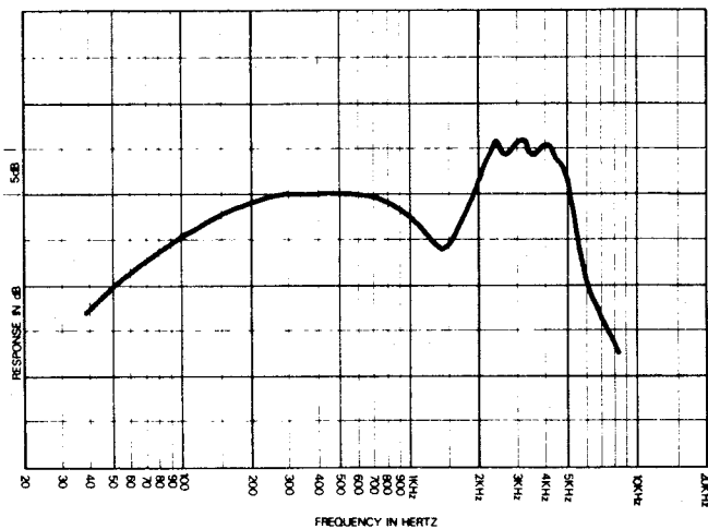
FIGURE 3 – Small Coil (1.75 in.) 12 in. Guitar Speaker
