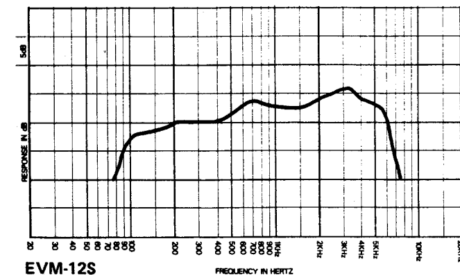
FIGURE 1 -- Frequency Response
