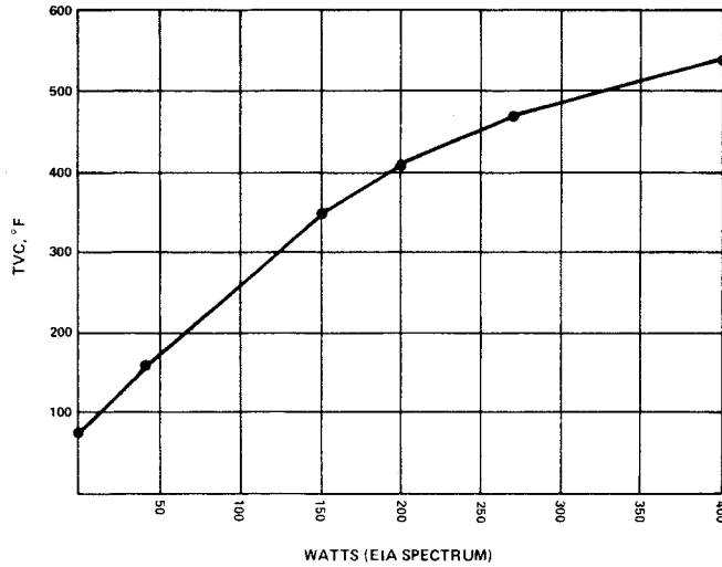
FIGURE 6 - Voice Coil Heat Rise
