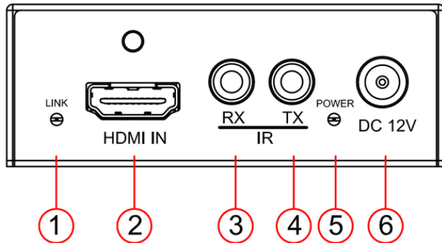
TD-TX2A-IR (Transmitter) Diagram
