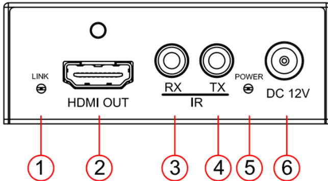
TD-RX2A-IR (Receiver) Diagram
